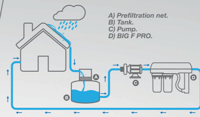
RAINWATER TREATMENT
